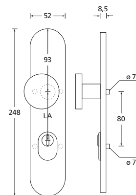
Cylinder projection: 11-16 mm
