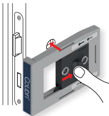
Drilling jig for key rosettes
